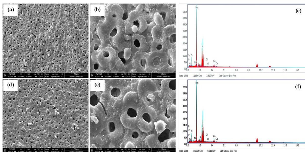
Fig. 12. The FE-SEM micrographs at two magnifications of 1000x and 5000x with EDS local analysis after exposure to SBF solution for 1 week for the coatings (a, b, c) without \text{Mg}_2\text{SiO}_4 NPs and (d, e, f) with \text{Mg}_2\text{SiO}_4 NPs.
