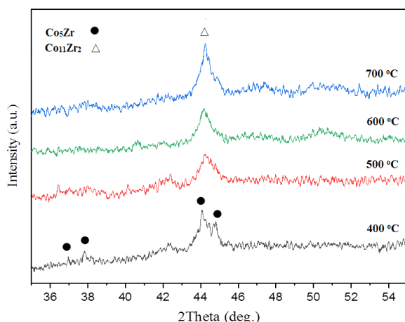
Fig. 5. The XRD patterns for melt-spun ribbons of \text{Co}_{78}\text{Zr}_{17}\text{B}_2\text{Si}_1\text{W}_2 alloys annealed at 400, 500, 600 and 700°C.
