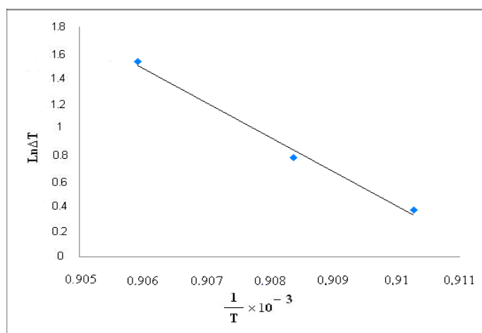
Fig 9. Variation of \text{Ln } \Delta T vs 1/T in \text{ST}_3\text{ZY}_1 for determination of the Avrami exponent according to Marotta method
