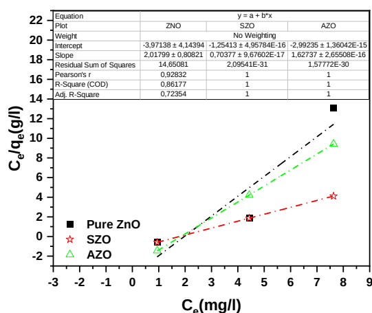
Fig. 14. Linearized Langmuir adsorption isotherms for Methylene Blue on ZnO-based thin films
