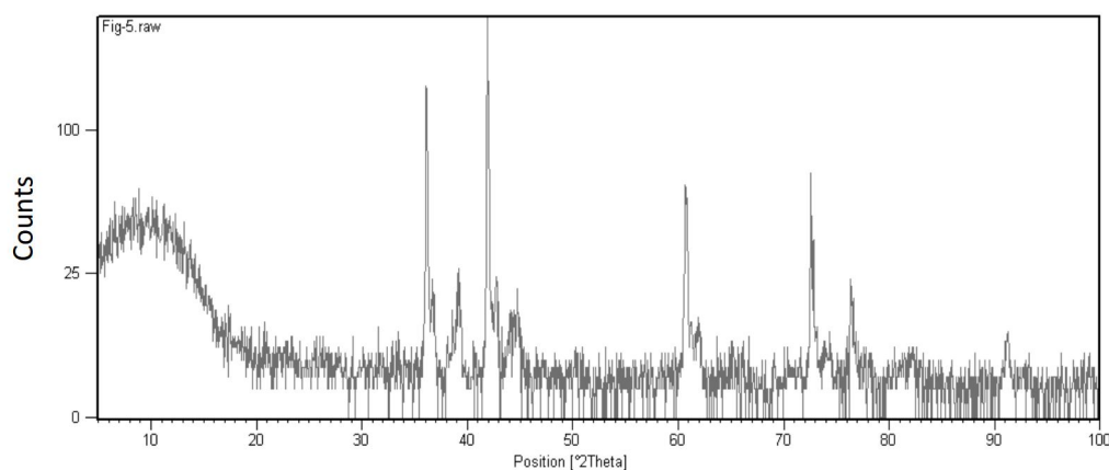
Fig. 5. XRD diagram of Activated and reacted Samples in microwave of 3\text{Ti}/\text{Al}/2\text{C} powder mixture
