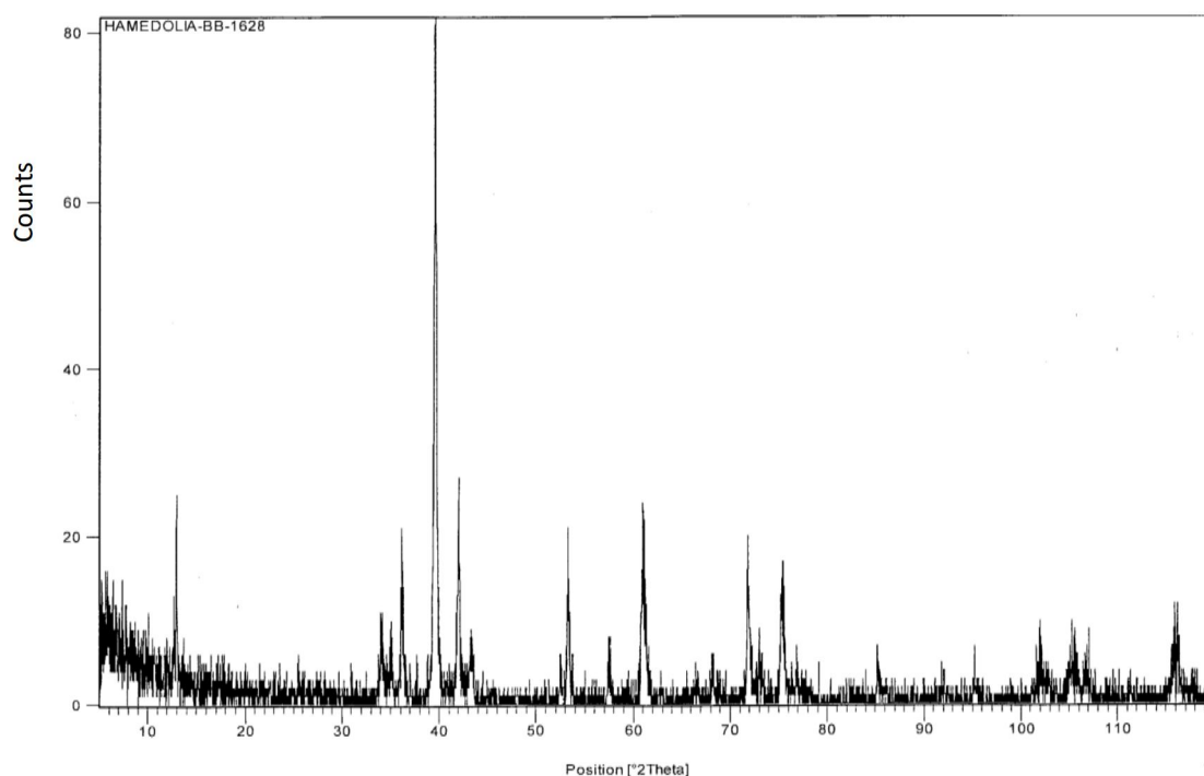
Fig. 4. XRD diagram of Activated and reacted Samples in microwave of 2\text{Ti}/\text{Al}/\text{C} powder mixture
