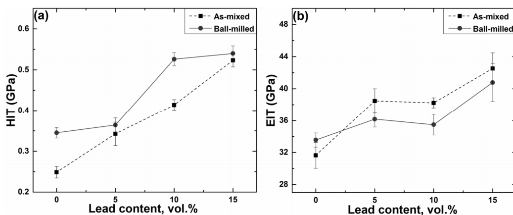
Fig. 4. Effect of varying lead content on the (a) Hardness and (b) Young modulus of sintered 6061Al alloys.
